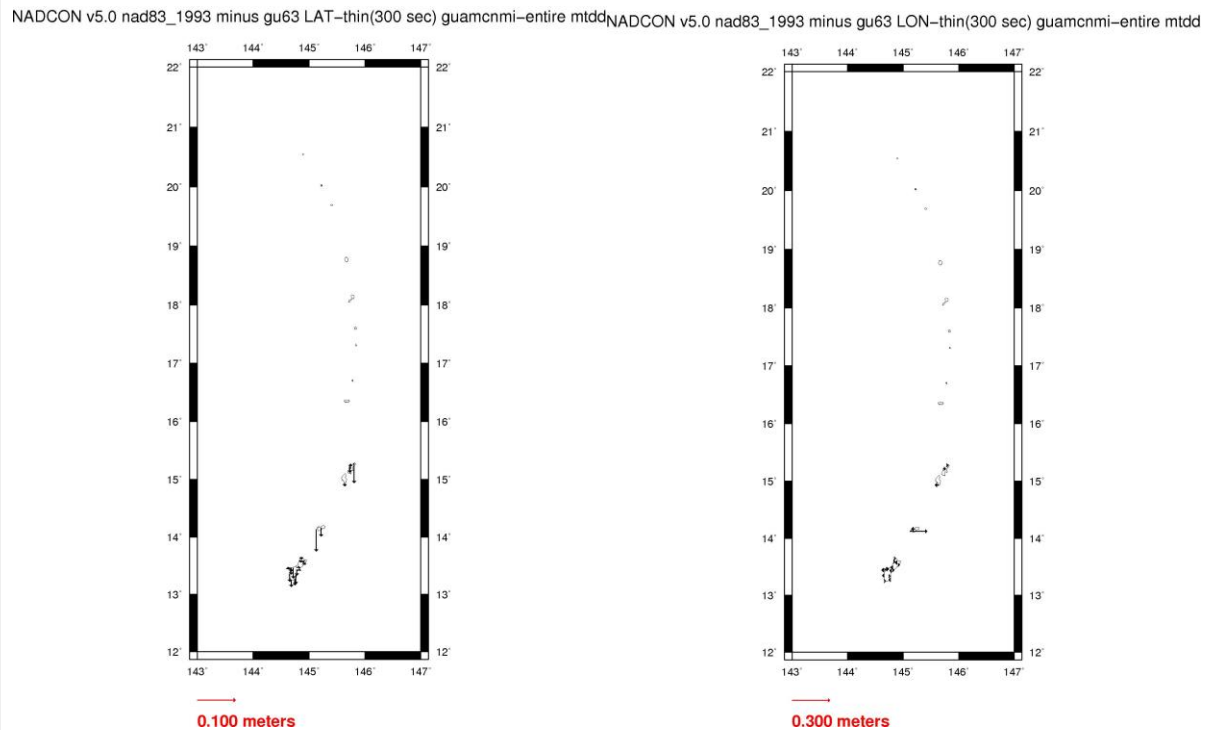
Figure 6-205: Thinned vector residuals (coordinate differences, minus the transformation grid), latitude (left) and longitude (right) components, in meters for GU63/NAD 83(1993)/Guam&CNMI.
