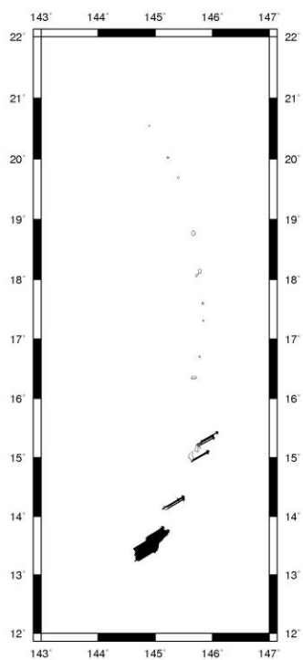
Figure 6-201: All horizontal vectors, GU63/NAD 83(1993)/Guam&CNMI.
