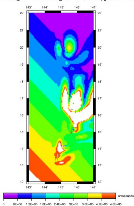
Figure 6-219: Errors for horizontal transformation, latitude (left) and longitude (right) components, in arcseconds for NAD 83(2002)/NAD 83(MA11)/Guam&CNMI.
