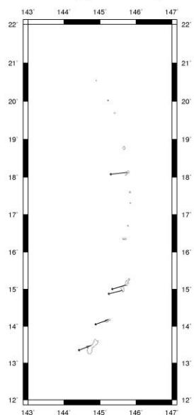
Figure 6-207: Thinned horizontal vectors after applying 15' grid spacing for NAD 83(1993)/NAD 83(2002)/Guam&CNMI.
