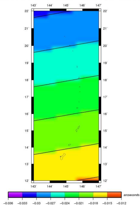
Figure 6-208: Horizontal transformation, latitude (left) and longitude (right) components, in arcseconds for NAD 83(1993)/NAD 83(2002)/Guam&CNMI.
