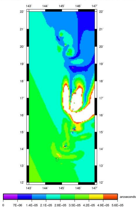
Figure 6-219: Errors for horizontal transformation, latitude (left) and longitude (right) components, in arcseconds for NAD 83(2002)/NAD 83(MA11)/Guam&CNMI.
