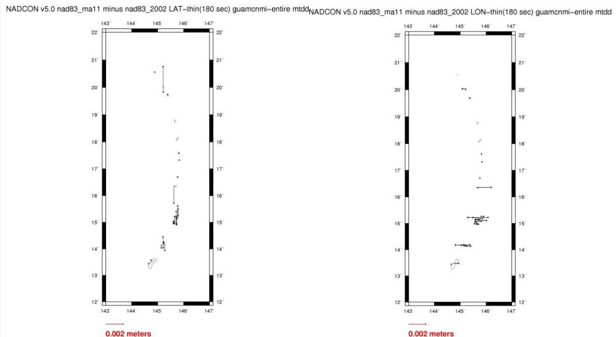
Figure 6-220: Thinned vector residuals (coordinate differences, minus the transformation grid), latitude (left) and longitude (right) components, in meters for NAD 83(2002)/NAD 83(MA11)/Guam&CNMI.
