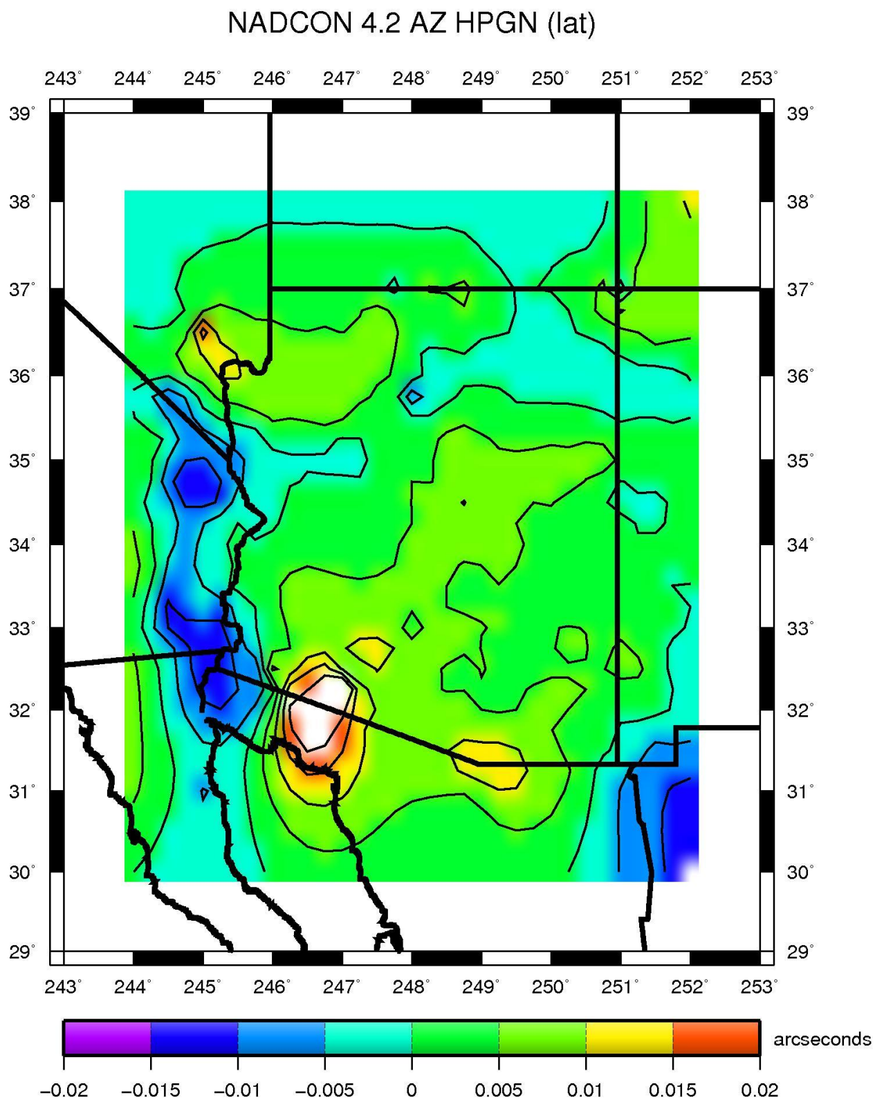
Figure 1-1: The Arizona HPGN latitude grid from NADCON 2.1 (and 4.2)
