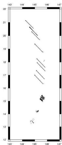
Figure 6-217: Thinned horizontal vectors after applying 3' grid spacing for NAD 83(2002)/NAD 83(MA11)/Guam&CNMI.
