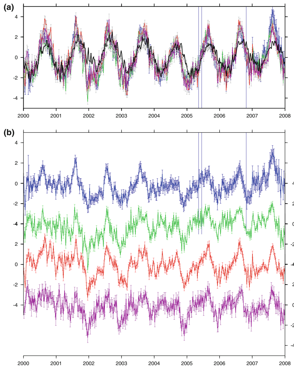
Fig. 2 a GPS scale variations for various ACs in color. Predicted scale of the loading model are shown in black . b Scale differences between GPS ACs and the loading model
